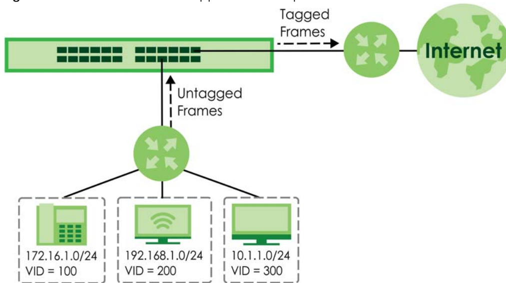
Figure 219 Subnet Based VLAN Application Example
