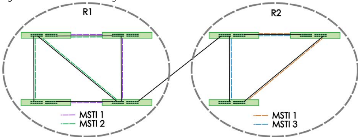
Figure 205 MSTIs in Different Regions
