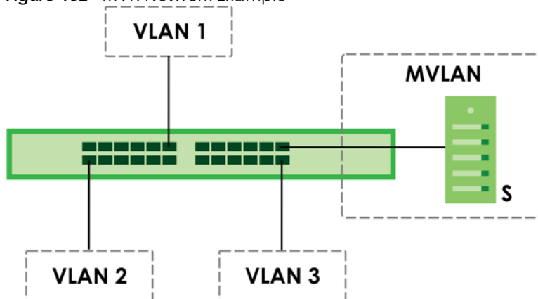
Figure 152 MVR Network Example
