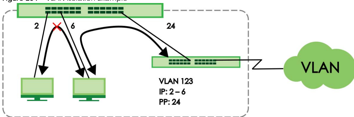
Figure 234 VLAN Isolation Example
