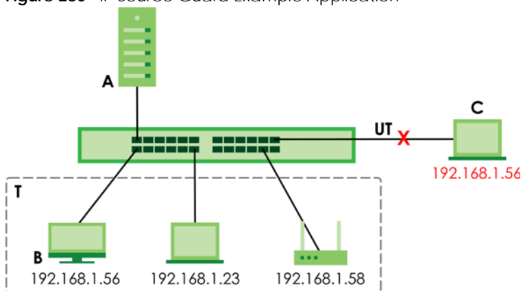
Figure 280 IP Source Guard Example Application
