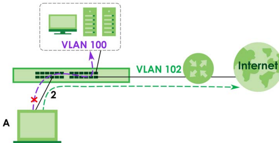
Figure 303 Guest VLAN Example
