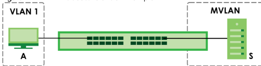
Figure 197 MVR Multicast Television Example
