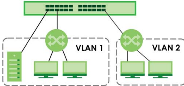
Figure 461 Shared Server Using VLAN Example
