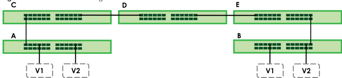
Figure 463 Port VLAN Trunking
