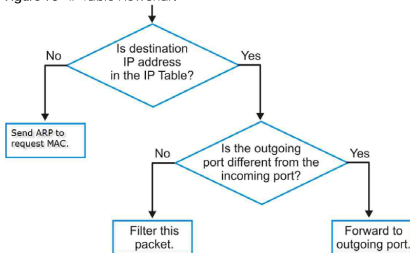
Figure 78 IP Table Flowchart
