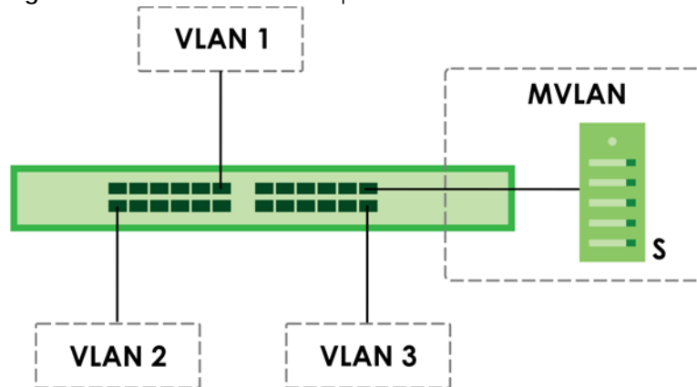
Figure 196 MVR Network Example
