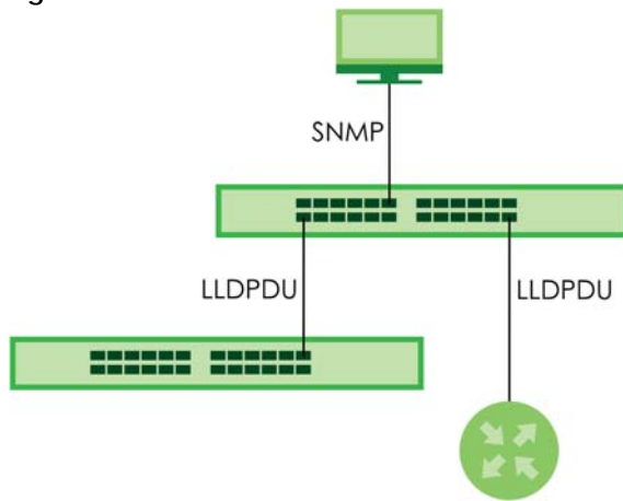
Figure 154 LLDP Overview
