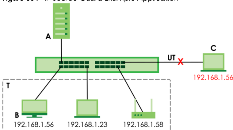
Figure 364 IP Source Guard Example Application
