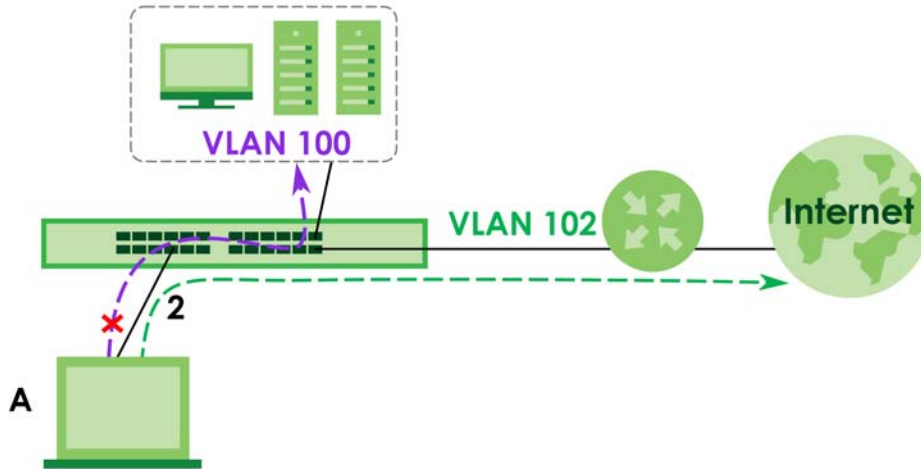
Figure 399 Guest VLAN Example
