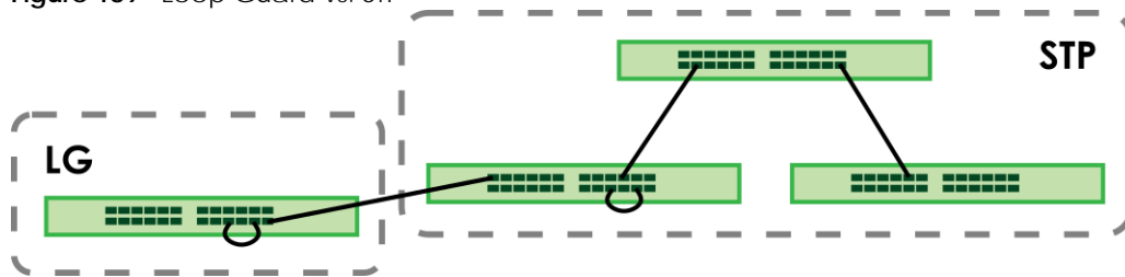
Figure 189 Loop Guard vs. STP
