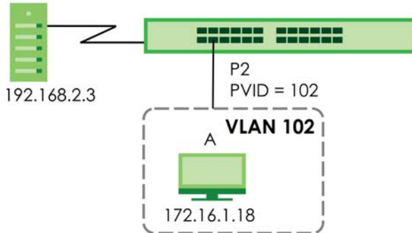
Figure 71 Getting Started: DHCP Relay Scenario
