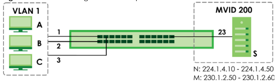
Figure 219 MVR Configuration Example
