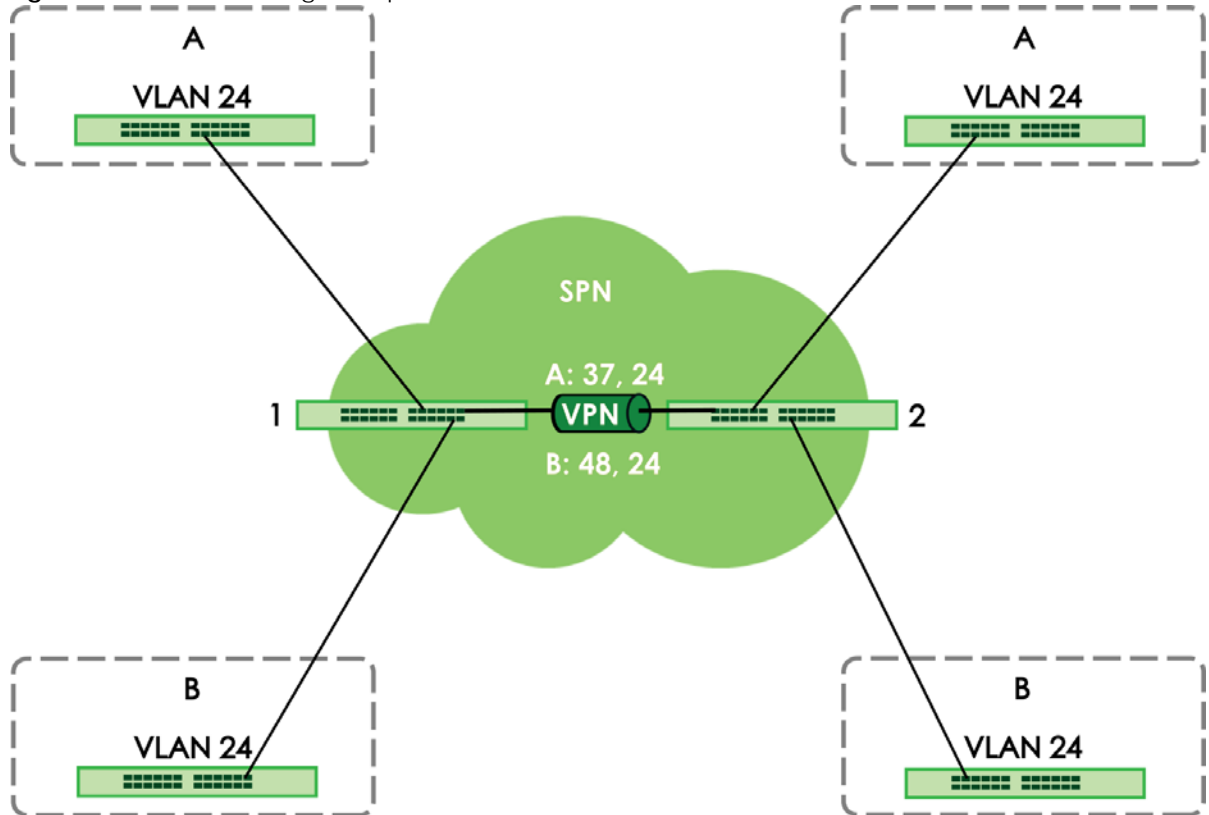
Figure 299 VLAN Stacking Example
