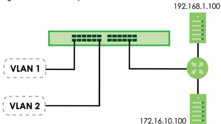
Figure 317 DHCP Relay for Two VLANs
