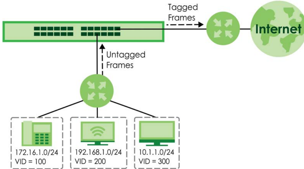
Figure 277 Subnet Based VLAN Application Example
