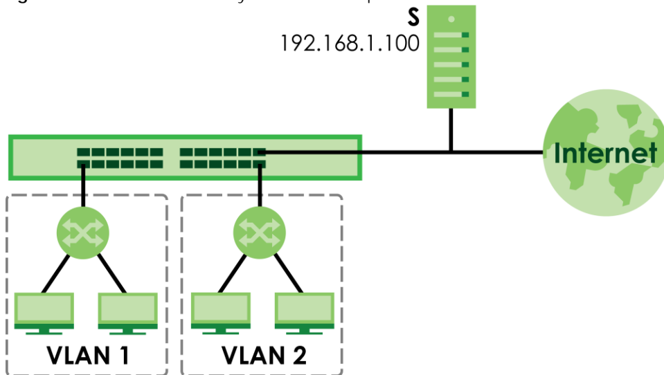
Figure 312 DHCP Smart Relay Network Example
