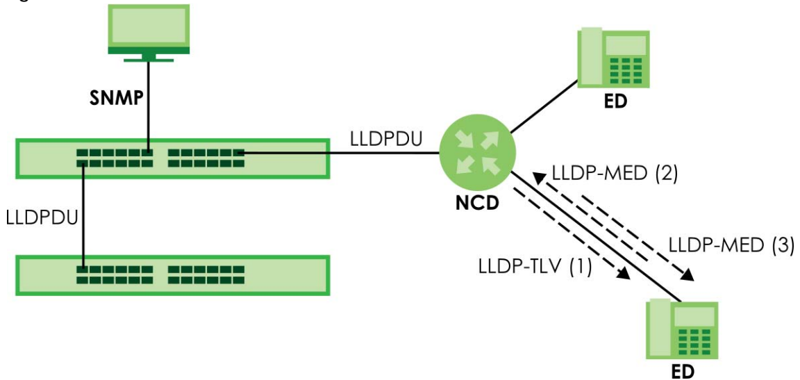
Figure 155 LLDP-MED Overview
