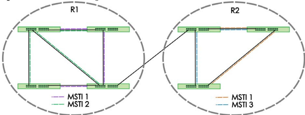
Figure 262 MSTIs in Different Regions
