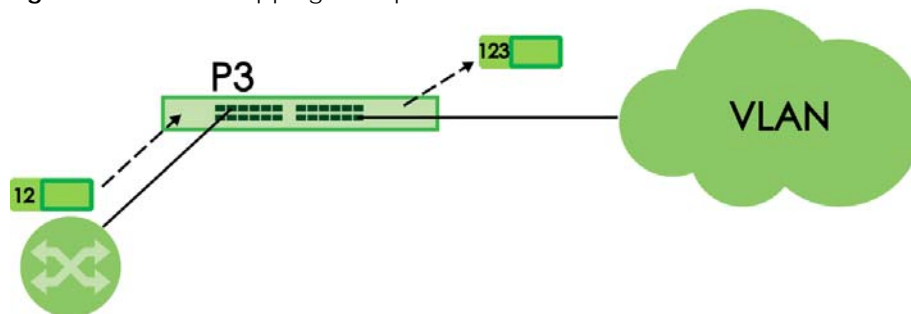
Figure 295 VLAN Mapping Example
