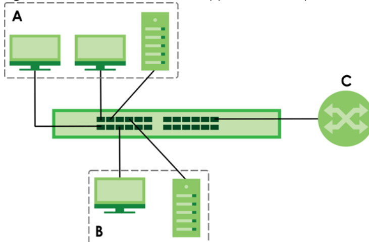
Figure 280 Protocol Based VLAN Application Example
