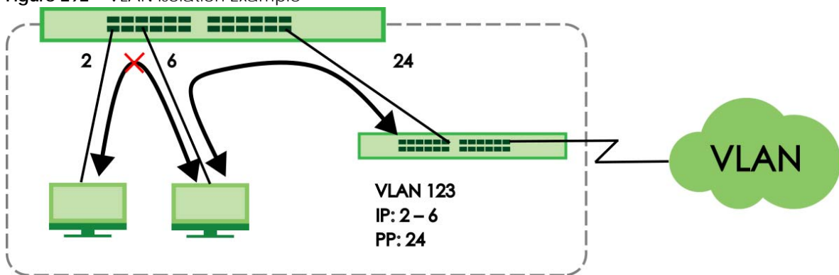
Figure 292 VLAN Isolation Example
