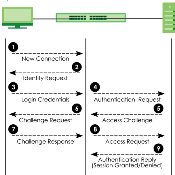
Figure 394 IEEE 802.1x Authentication Process
