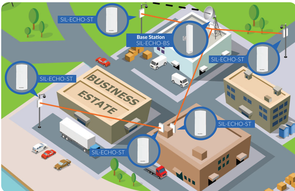
SIL-ECHO-BS as a Base Station in PtMP & SIL-ECHO-ST as the station (CPE) & PtP link
