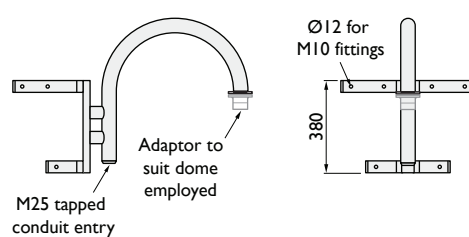
C-1699/F Corner mount
