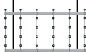
Ceiling Mount for INFILED WP Series 5x5 DVLED Videowall
