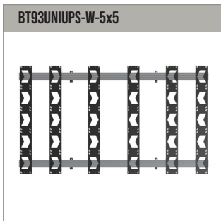
Wall Mount for Unilumin UpanelS Series 5x5 DVLED Videowall
