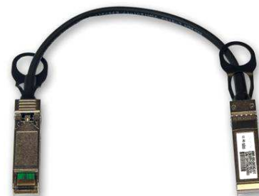
SIL-10G-DATAC-XX 10Gbps SFP+ Direct Attach Cable (DAC)
